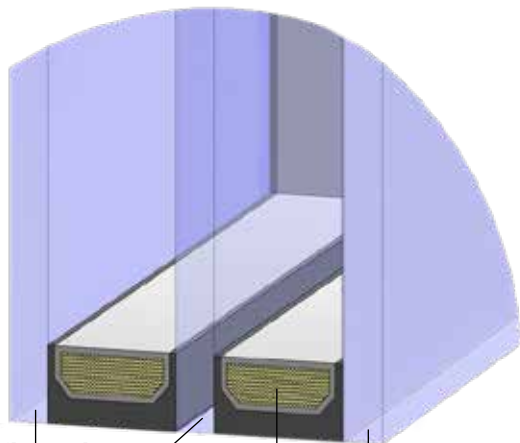
4mm float glass 4mm float glass 4mm float glass Insulated Spacer 12-36mm
