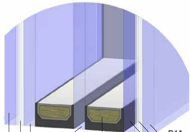
P4A 4mm glass 4 tapes 4mm glass 4mm float glass Insulated Spacer 12-36mm P4A 4mm glass 4 tapes 4mm glass
